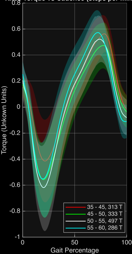
Knee Torque vs Cadence (steps per minute)
