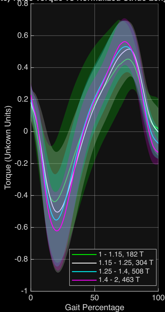
Knee Torque vs Normalized Stride Length
