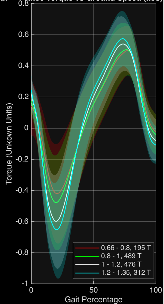
Knee Torque vs Ground Speed (m/s)
